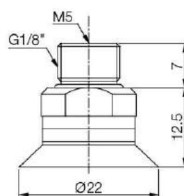
[With M518MFO fitting]
